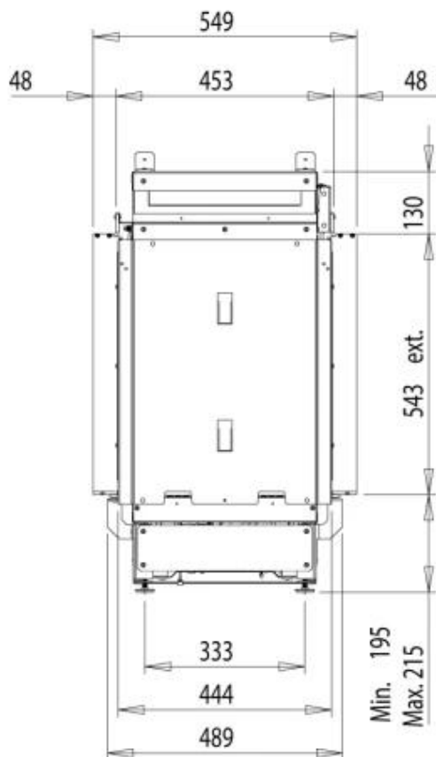
Dimensional Drawing e-Matrix heat 800x500 ST (MkII)
